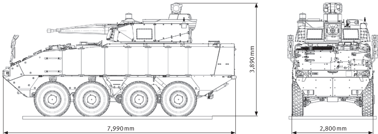
Integration of Oerlikon Skyranger® 30 shown on GDELS-Mowag Piranha 4
