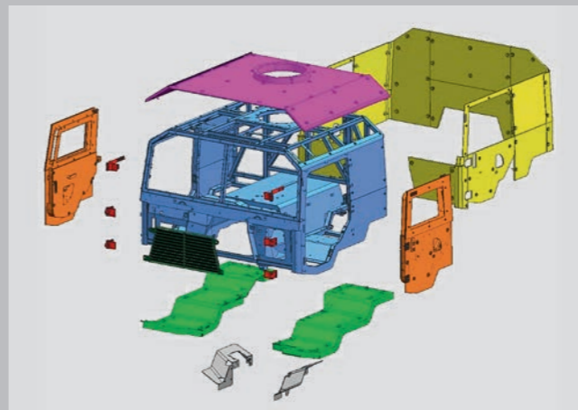
Concept C – Modular Space Frame with Integrated Armour Kit
