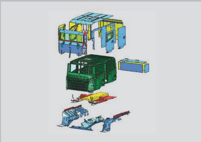
Concept A – Soft Skin Cabin with Armour Kit as Stand-alone inside Cabin
