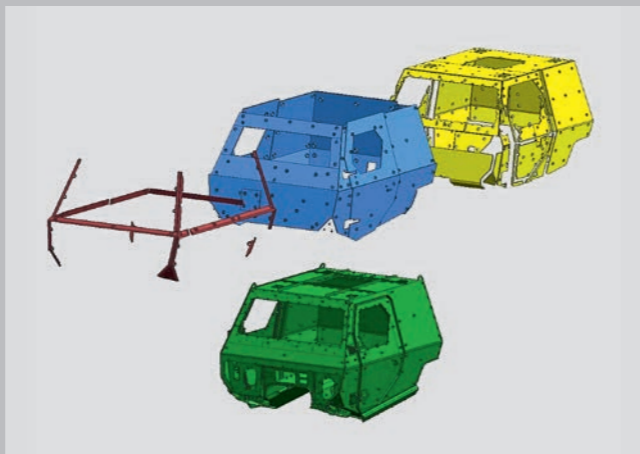
Concept B – Steel Cabin with Add-on-Armour for ballistic and mine/IED protection
